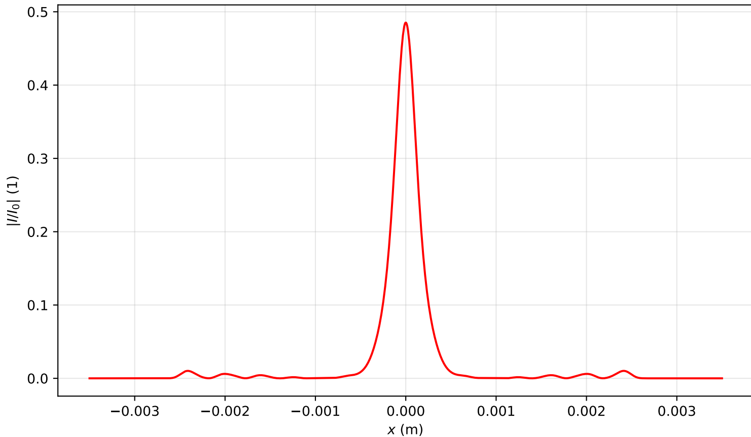
Intensity profile I(x, y = 0, z = 2.548)/I_0 , P_{in}=7.0P_{cr} , artificial time
